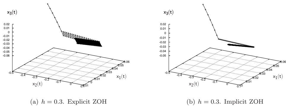
Figure 8: Equivalent control based SMC, Trajectory with initial point x_0 = [0.05, -0.5, 0.02]
