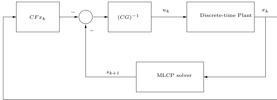
Figure 3: Control system schema with implicit Euler implementation.
