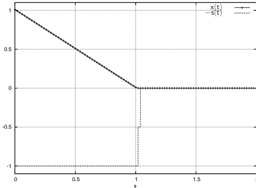
(b) State and Control vs. Time h = 0.02
