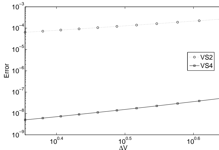
Figure 5: Log-Log plot of the error on the first spike timing as a function of the voltage-step. Circles and squares are voltage-stepping methods with a piecewise linear interpolation at the boundaries of the voltage-interval (VS2) and at the gaussian abscissas (VS4), respectively. The lines (not fits) indicate the order of the methods. Dotted-line is second order and solid-line is fourth order.
